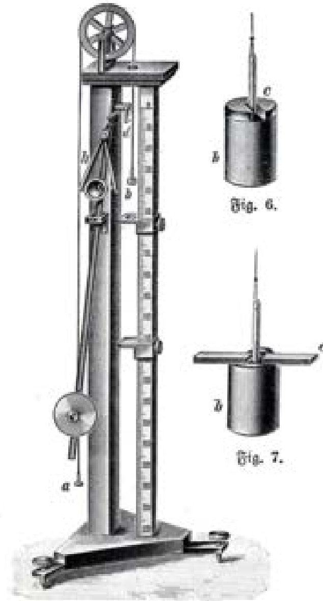
Fig. 6. Atwood's Ball Machine
